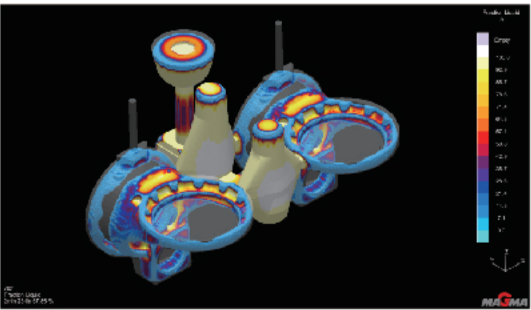
Liquid-phase ratio during solidification/cooling
